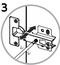
Side adjustment / Ajuste lateral
